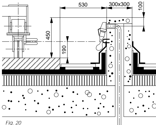
Fig. 20 Power point on concrete track support plinth
